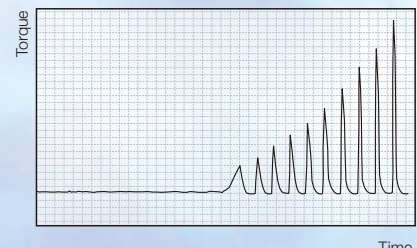
Impact Mode Torque Curve
